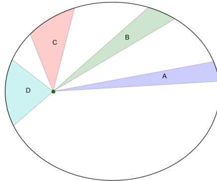
Figure 1: Computer-modeled elliptical orbit
